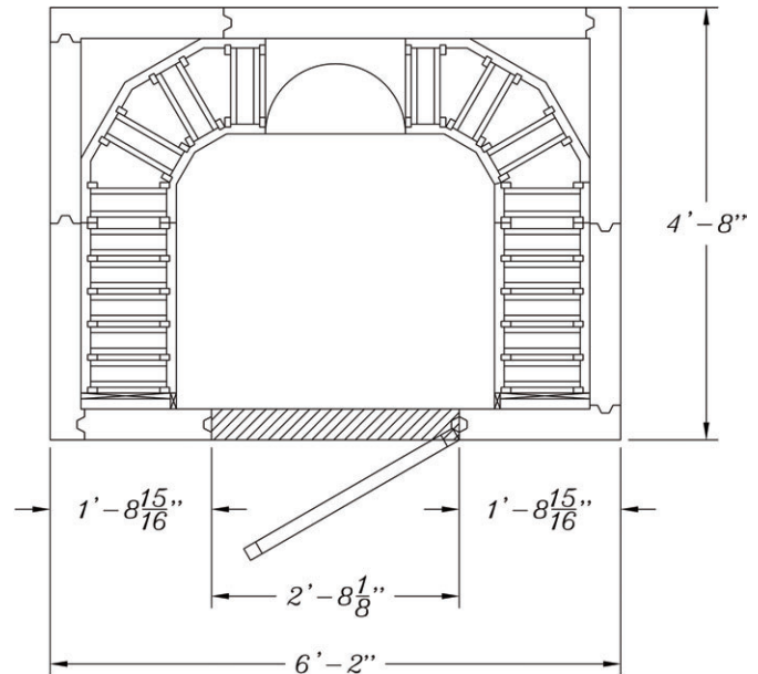
Standard Wine Locker Drawing
